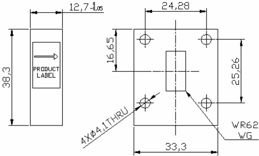
All units in mm
